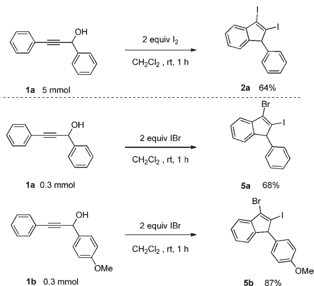
Scheme 2. Synthesis of Functionalized Indenes
